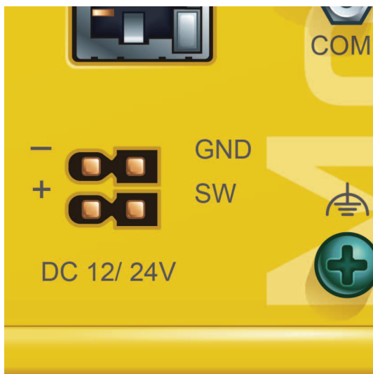
Fig. 6: Terminals of NoriGate V2
