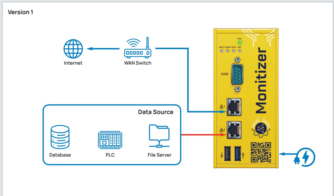
Fig. 15: NoriGate V1 : Initial connection without further troubleshooting
