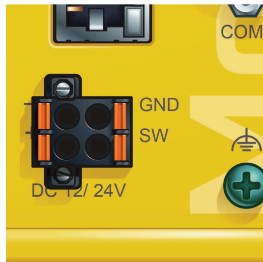
Fig. 7: Terminal pin adaptor NoriGate v2
