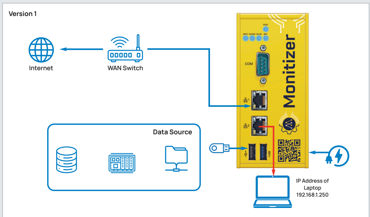
Fig. 16: NoriGate V1 : Connection for further troubleshooting
