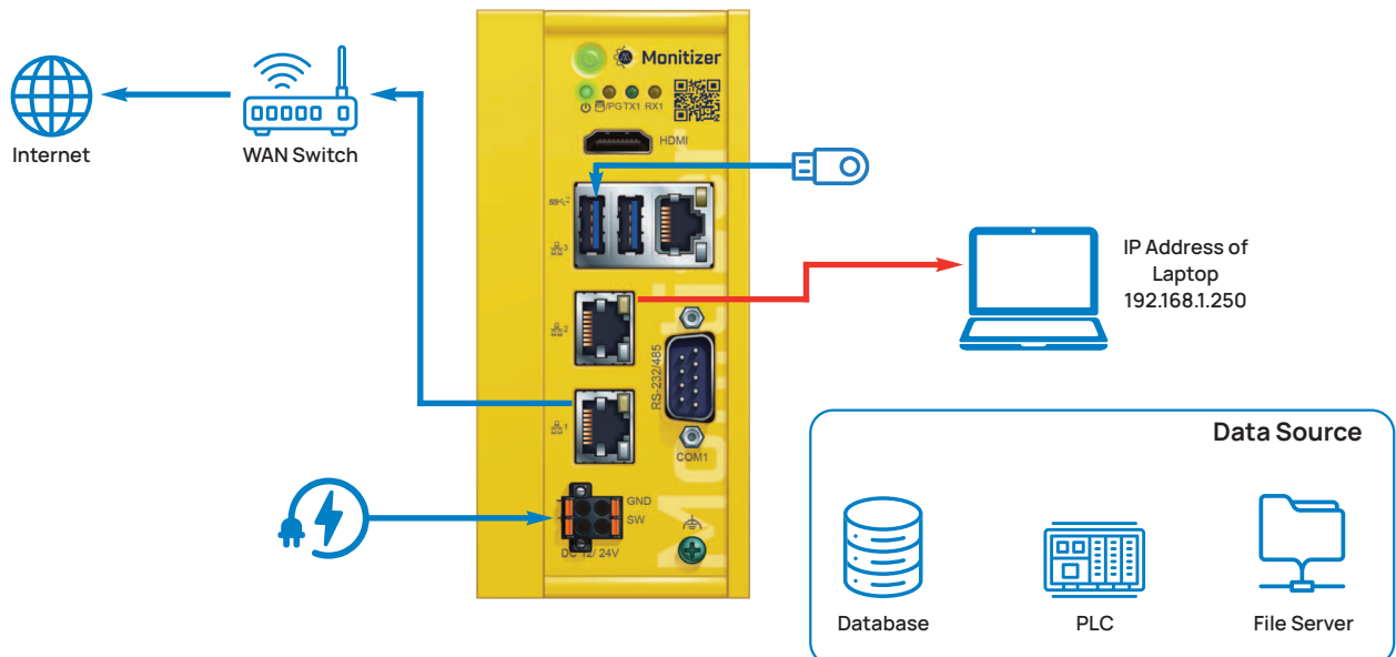
Fig. 18: NoriGate V2 : Connection for further troubleshooting
